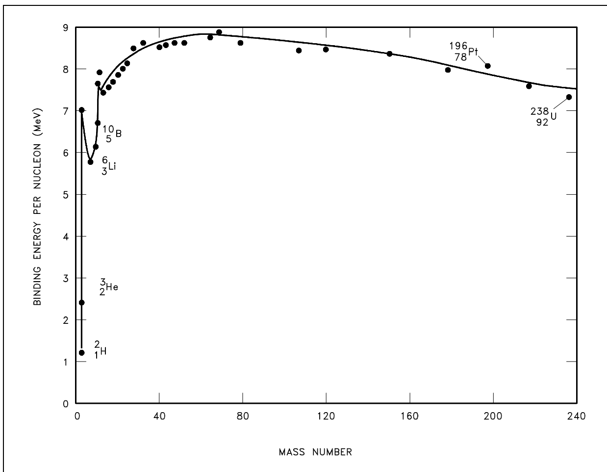
Figure 20 Binding Energy per Nucleon vs. Mass Number
